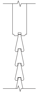
OPTIONAL CHEVRON NON-VENTED LOUVER Available in 1-3/4" only
